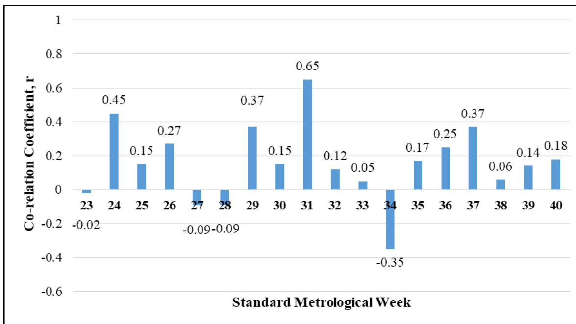
Figure 3. Correlation between weekly rainfall and yield
