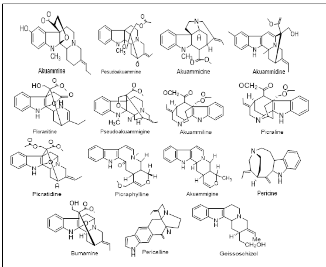
Figure 1. Chemical structures of alkaloids isolated from P. nitida
