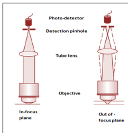
Figure 2. The principle of confocal fluorescence microscopy Light coming from out-of-focus planes is largely blocked by a pinhole in front of the detector
