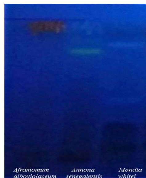
Figure 8. TLC Chromatogram of methanolic extracts of studied plants without controls at 366 nm
