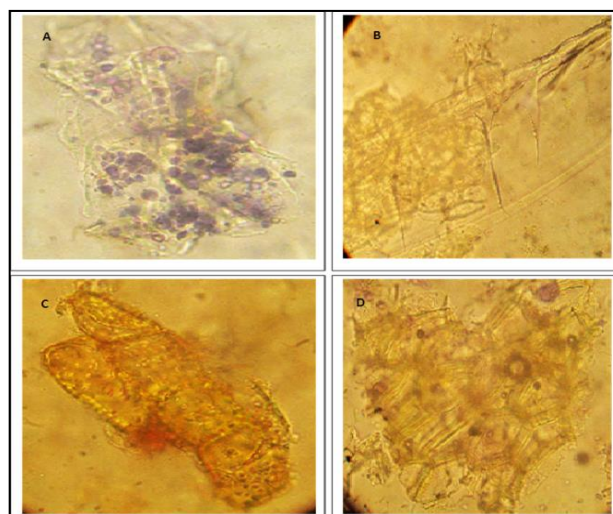
Figure 5. Microscopic features of M. whitei , (A) starch grains (B) fiber fragments (C) beam fragments (D) parenchyma
