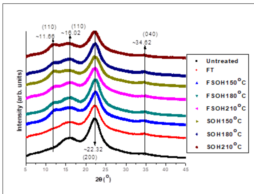
Figure 2. X-ray diffractogram of untreated and freeze-silicone oil heat treated wood
